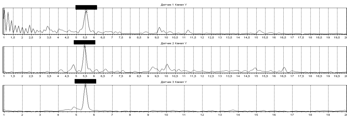
Figure 5. The spectrum of vibrations along the Y axis. The appearance of dangerous low-frequency vibrations during the passage of a freight train on a landslide-prone section in Ulyanovsk city
